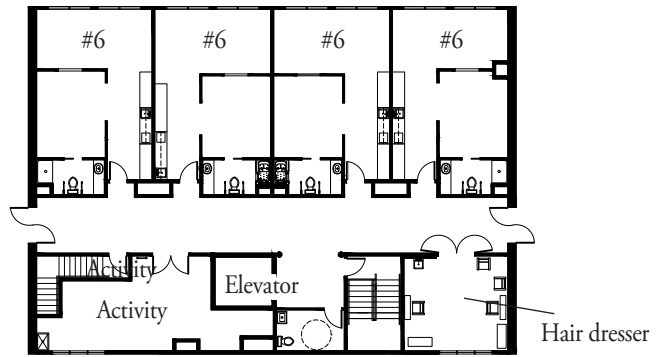
SECOND FLOOR CORE
